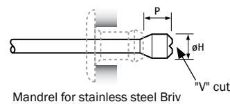
Mandrel for stainless steel Briv
